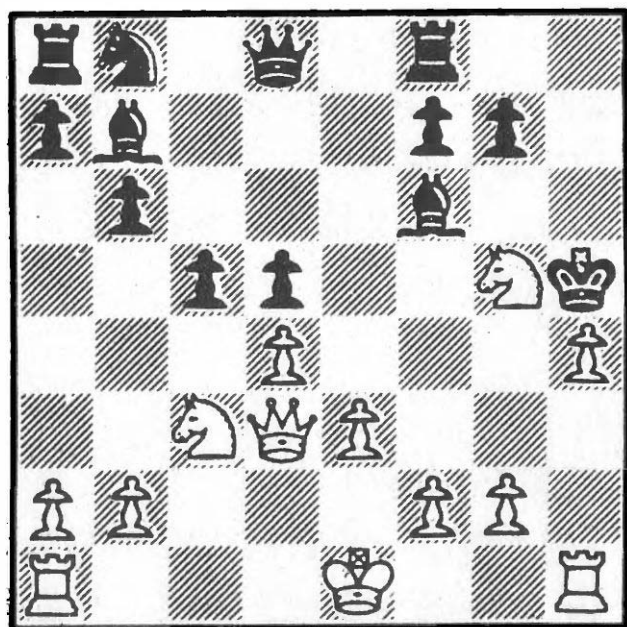
454 After 13...Kh5
